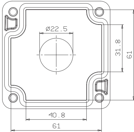
Kapak / Cover
