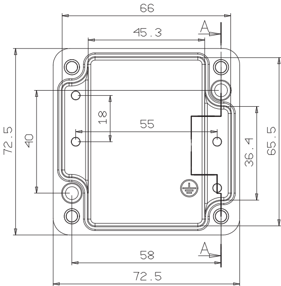
Gövde / Housing
